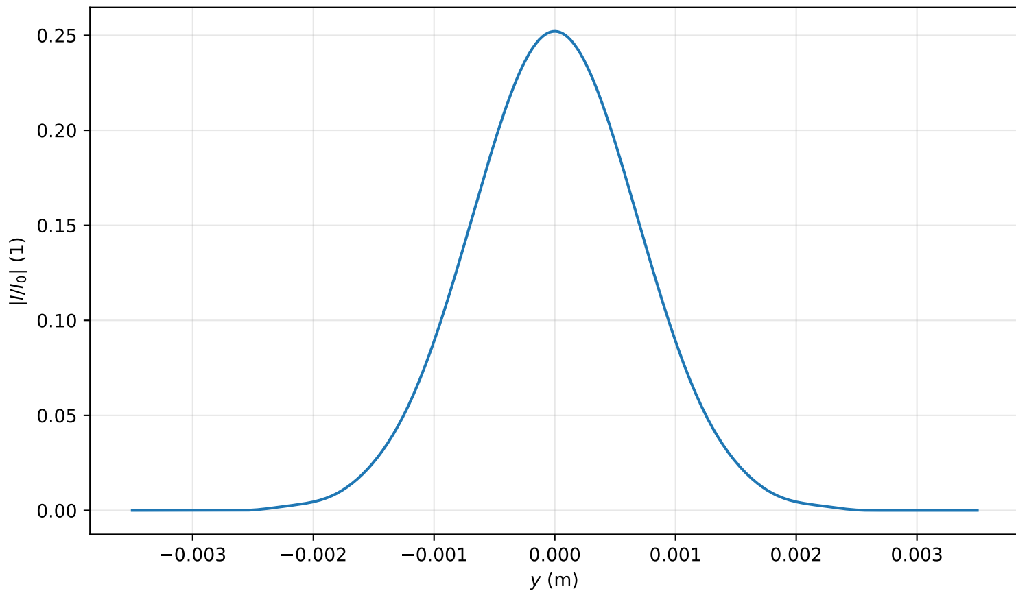
Intensity profile I(x=0, y, z=3.662)/I_0 , P_{in}=0.1P_{cr} , artificial time
